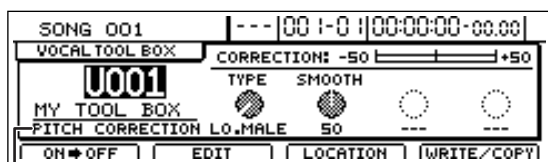
Algorithm name
